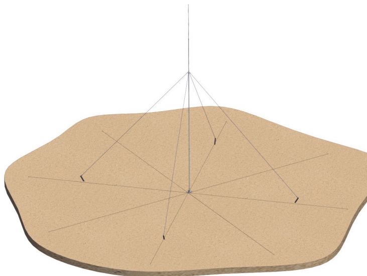
LB009 shown with LA003 earth mat
