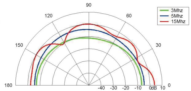
Elevation at 90°
