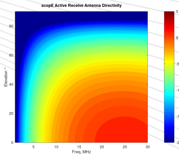
Figure 2 – Radiation Pattern Modelled above perfect ground
