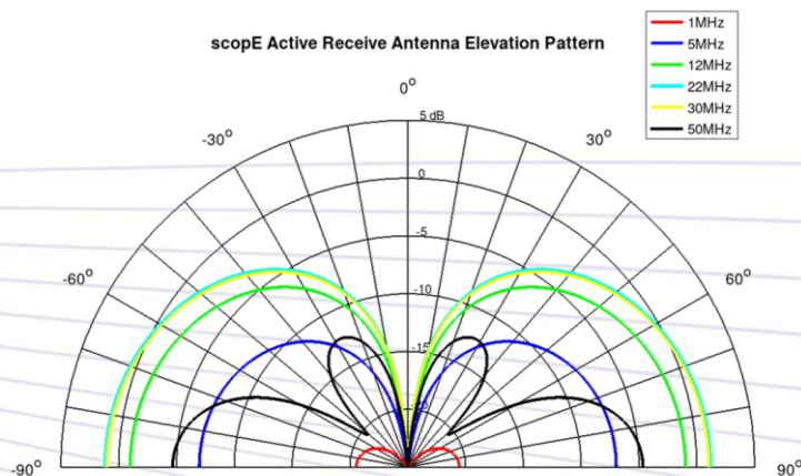
Figure 2 – Radiation Pattern Modelled above perfect ground
