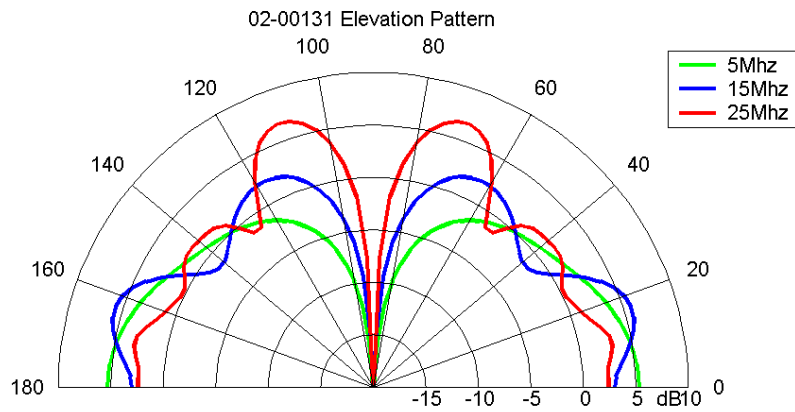
Figure 2 – Radiation Pattern
