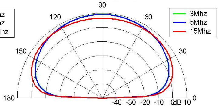
Figure 4 – Elevation at 0°
