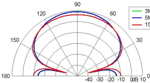
Figure 3 – Elevation at 90°
