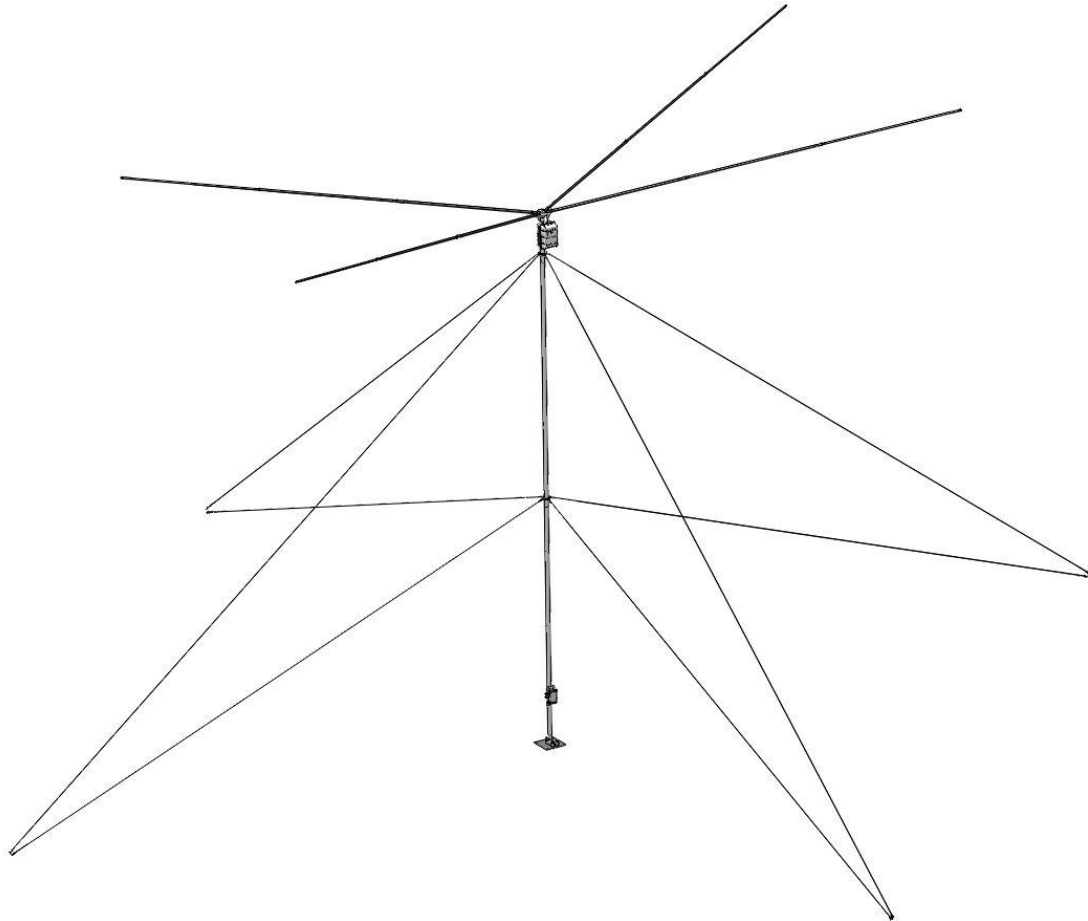
Figure 1 – 02-00131 Installed Antenna
