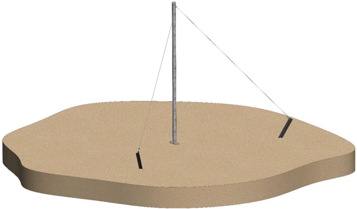
Figure 1 – Stub Mast Installed
