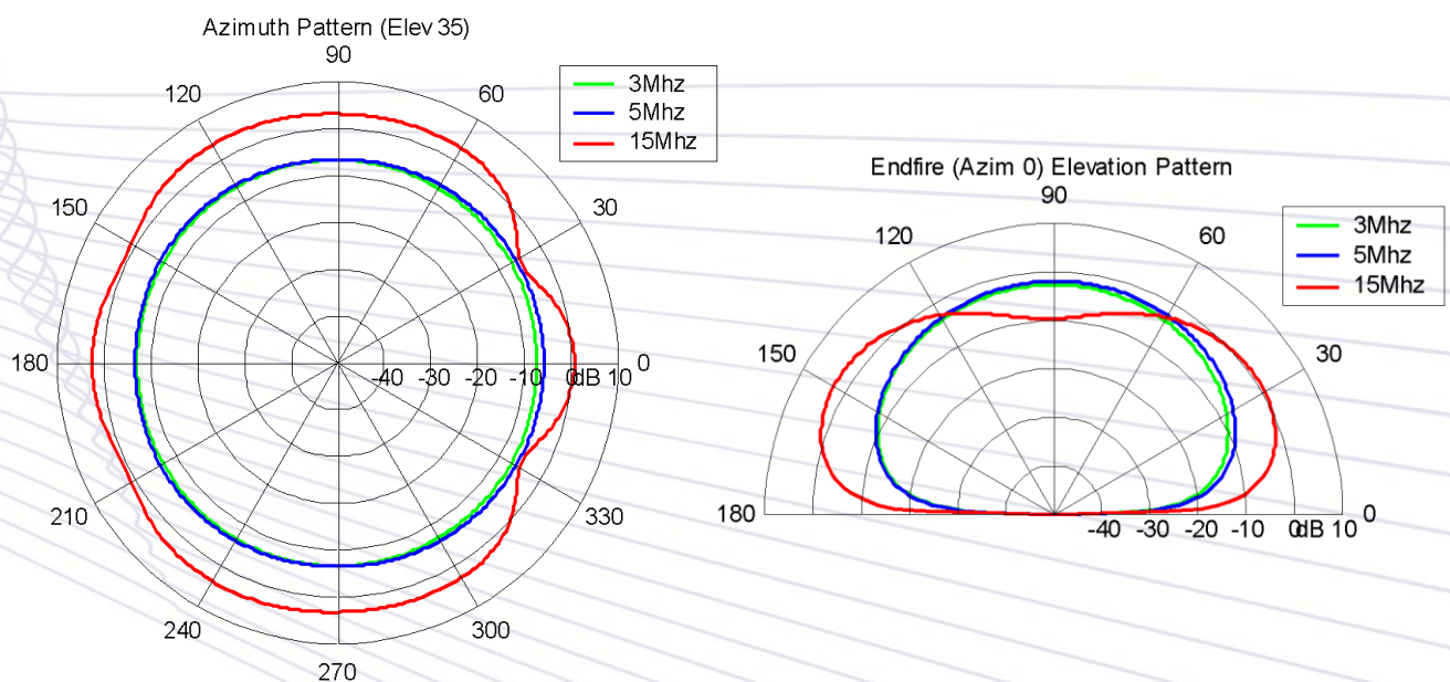
Figure 2 – Radiation Patterns
