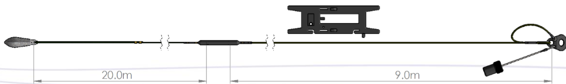
Figure 3 - Antenna Dimensions
